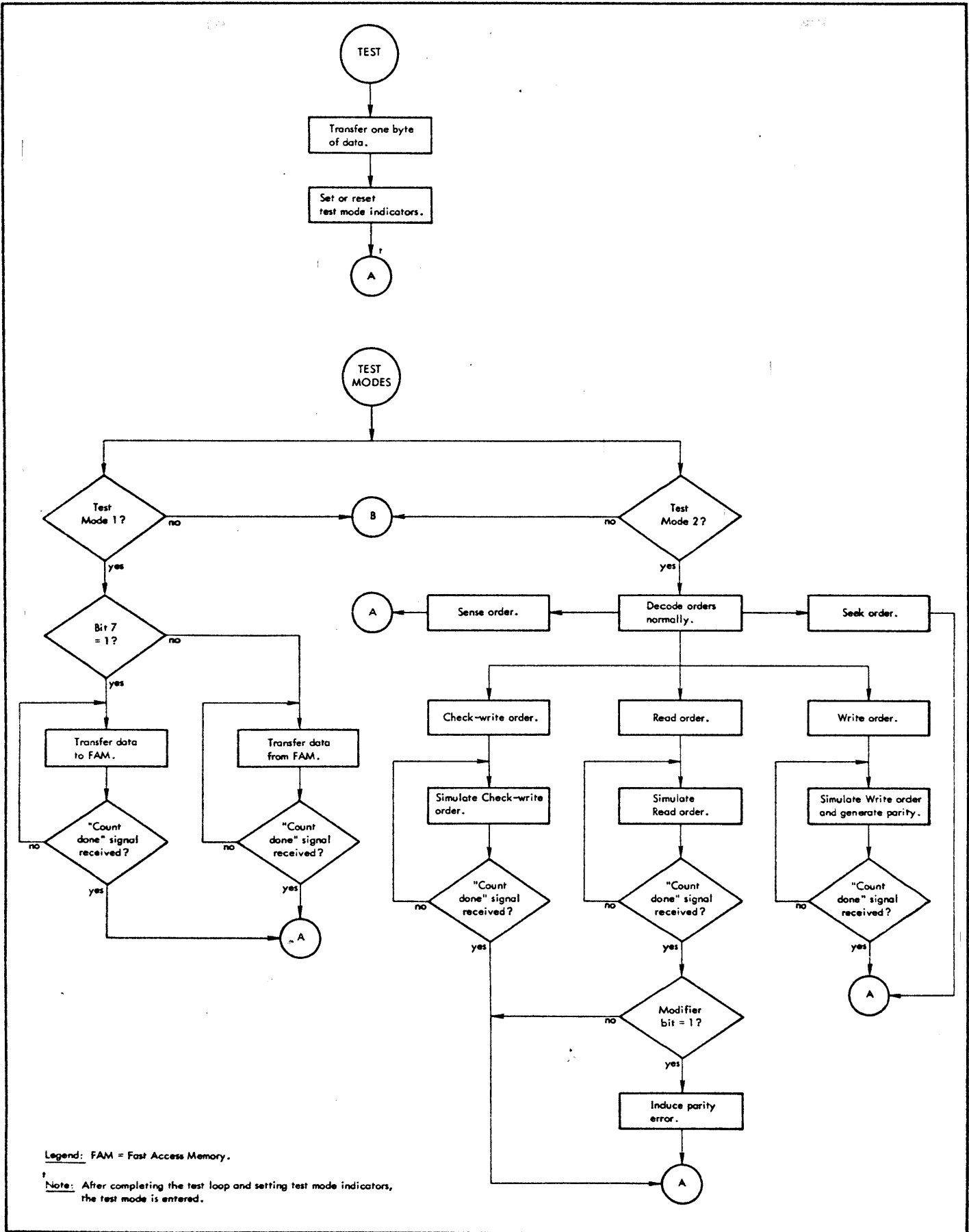
Figure 13. Test Order
