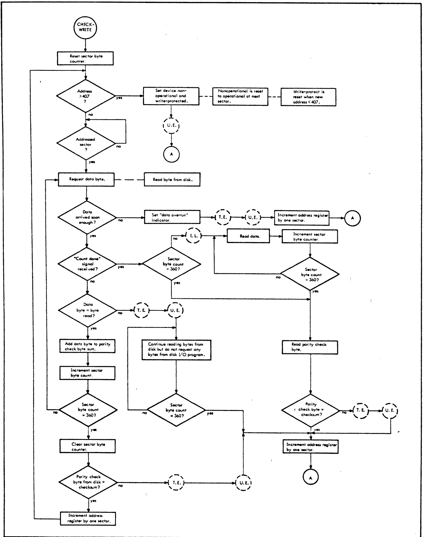
Figure 12. Check-write Order
