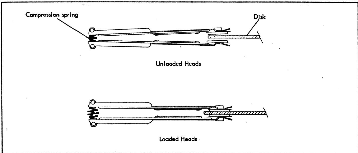
Figure 3. Read/Write Heads
