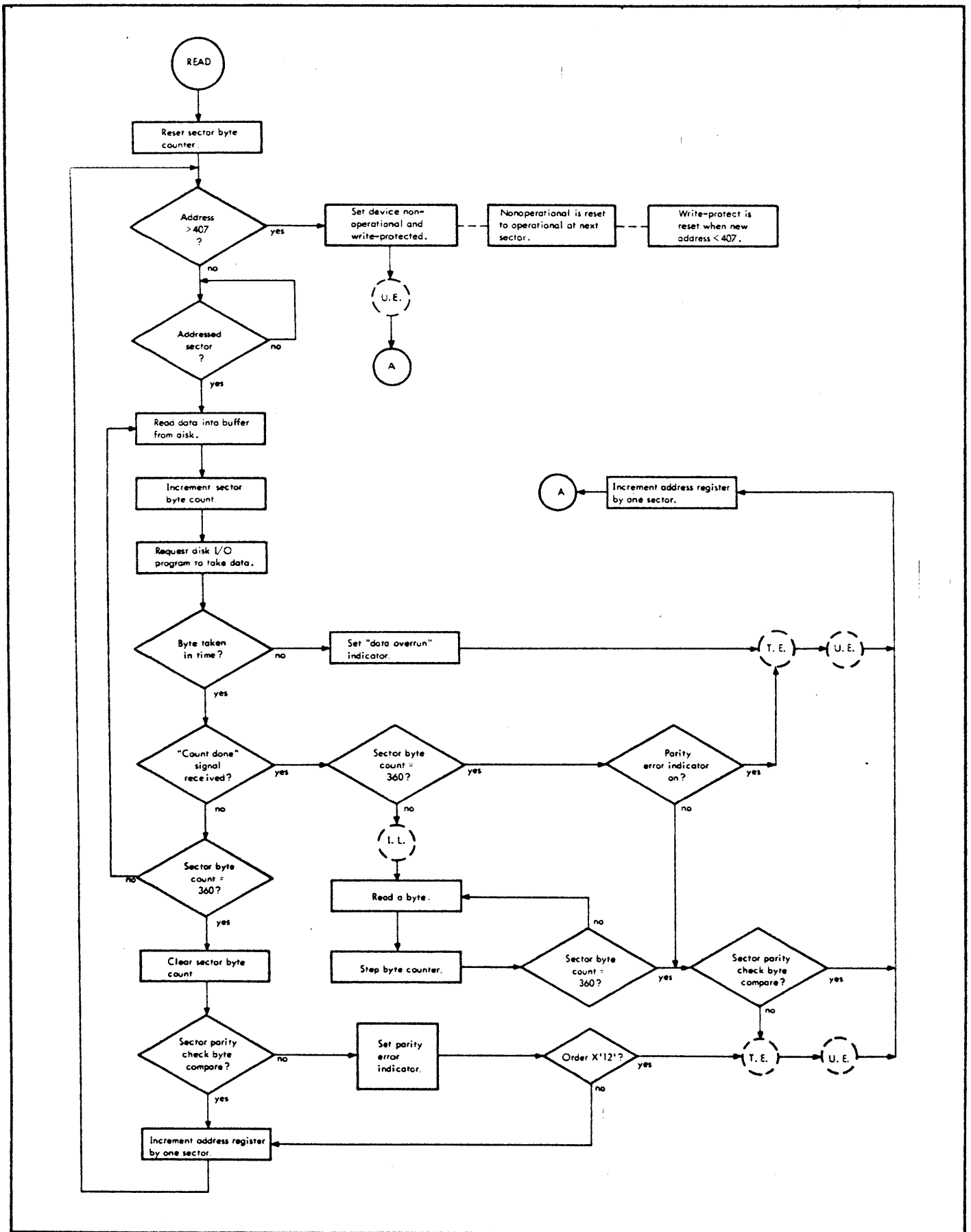
Figure 10. Read Order
