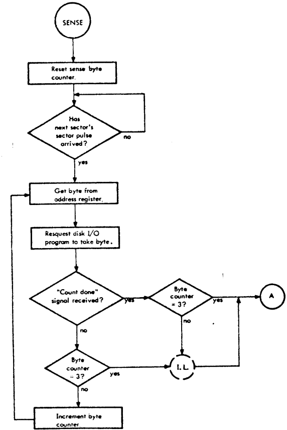
Figure 11. Seek/Sense Order
